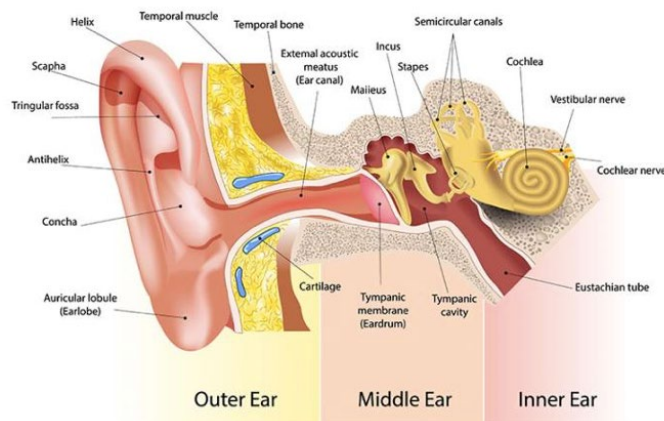
Figure 1 ("Ear Anatomy")
